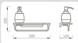
WY89610A SHELF + SOAP DISPENSER WITH TOWEL RING MATERIAL : BRASS+GLASS FINISHING : CHROME
