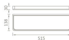
SP-68003A SHELF 515x138MM MATERIAL : BRASS FINISHING : CHROME
