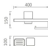
S401708A 4WAY = SHELF + SOAP DISH + TUMBLER HOLDER + TOWEL RING SIZE: 400x100x23x19 MATERIAL : BRASS+GLASS FINISHING : CHROME
