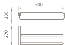
SB-75102 TOWEL RACK 600MM MATERIAL : BRASS FINISHING : CHROME
