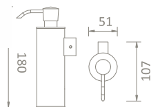
AN-95014 SOAP DISPENSER MATERIAL : BRASS FINISHING : CHROME
