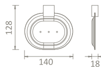
AN-95011 SOAP DISH MATERIAL : BRASS FINISHING : CHROME
