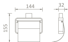
AN-95008 PAPER HOLDER WITH COVER MATERIAL : BRASS FINISHING : CHROME
