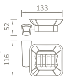
SB-75007A SOAP HOLDER MATERIAL : BRASS+GLASS FINISHING : CHROME
