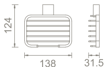
AN-95010 SOAP DISH BASKET MATERIAL : BRASS FINISHING : CHROME
