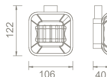
AN-95002A SOAP HOLDER MATERIAL : BRASS+GLASS FINISHING : CHROME
