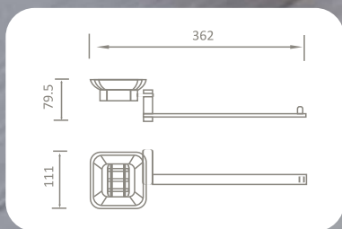
OS-10106A SOAP HOLDER WITH NAPKIN RING MATERIAL : BRASS+GLASS FINISHING : CHROME
