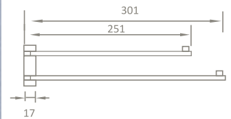
OS-10104 DOUBLE SWIVEL TOWEL BAR MATERIAL : BRASS FINISHING : CHROME
