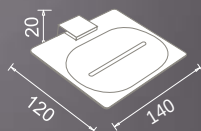
K-71009 FORGING SOLID SOAP DISH MATERIAL : BRASS FINISHING : CHROME
