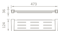
SB-75103 SHELF WITH FRAME 473x124MM MATERIAL : BRASS FINISHING : CHROME
