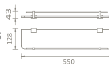
AN-95015A SHELF 550x128MM MATERIAL : BRASS+GLASS FINISHING : CHROME
