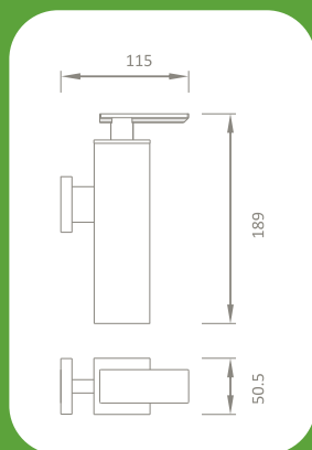
OS-10101 SOAP DISPENSER (USA MODEL) MATERIAL : BRASS FINISHING : CHROME
