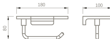
WY89210 SHELF WITH PAPER HOLDER MATERIAL : BRASS FINISHING : CHROME
