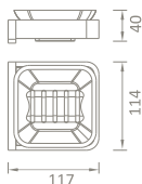
SP-68007A SOAP HOLDER MATERIAL : BRASS+GLASS FINISHING : CHROME
