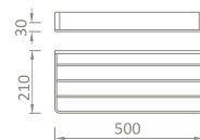
SP-9418 DOUBLE TOWEL RACK 500MM MATERIAL : BRASS FINISHING : CHROME
